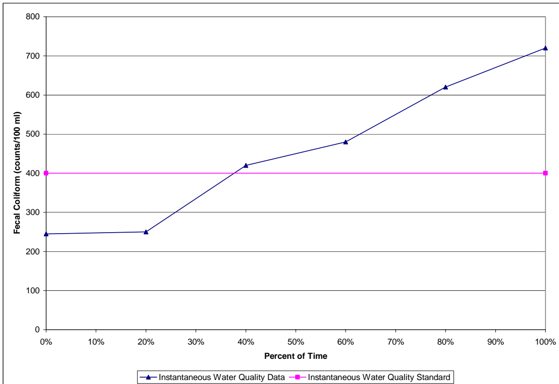
Figure 5. 10% Test Curve for Station PAN1-6, Summer 2005
