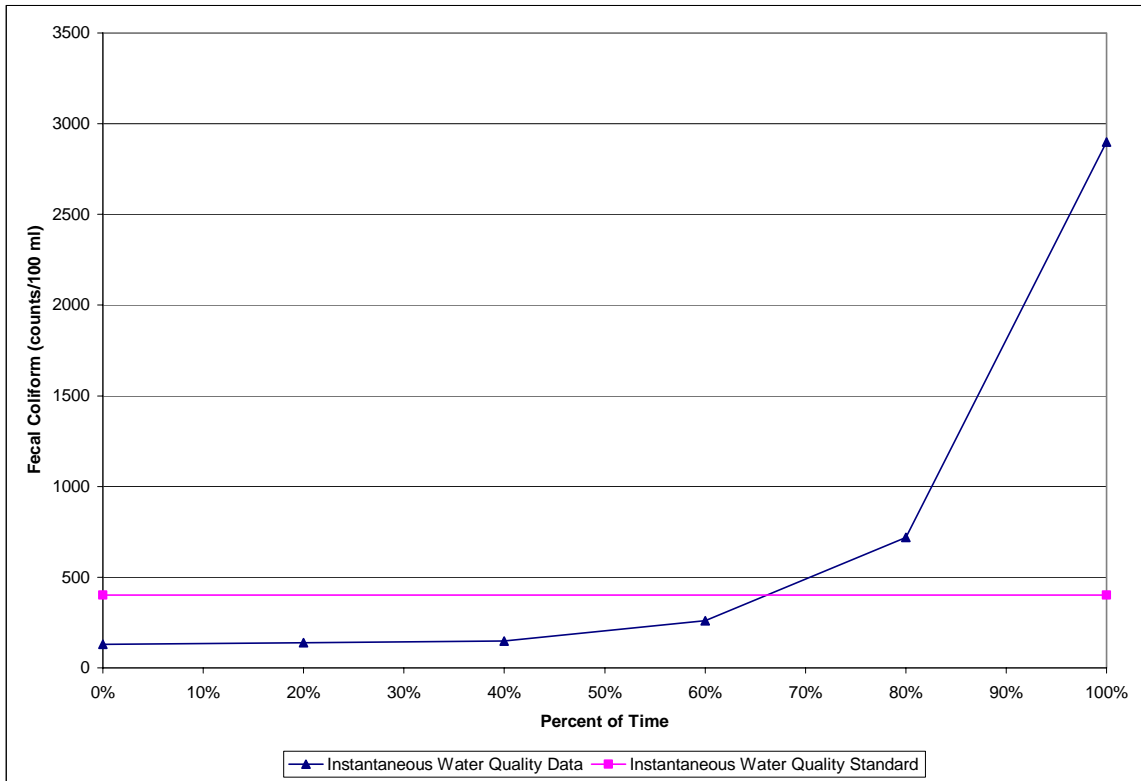
Figure 6. 10% Test Curve for Station PAN1-6, Summer 2006
